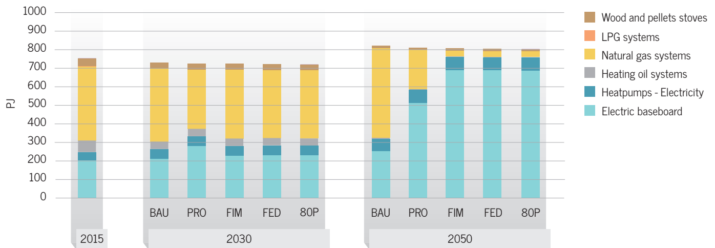
Figure 4.8 – Space heating systems in the residential sector
