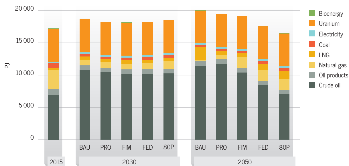
Figure 5.2 – International exports
