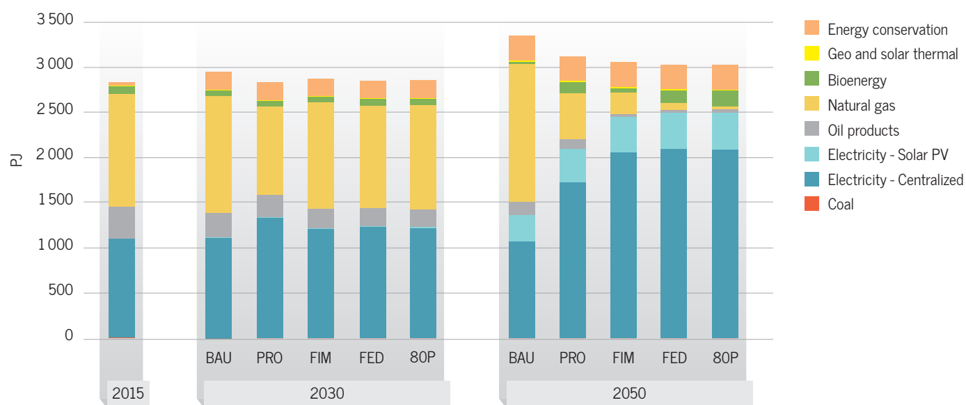
Figure 4.4 – Final energy consumption in residential, commercial and agricultural sectors
