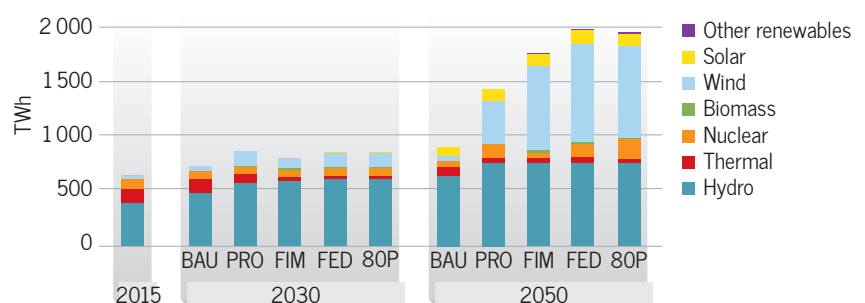
Figure 4.2 – Electricity generated by source
